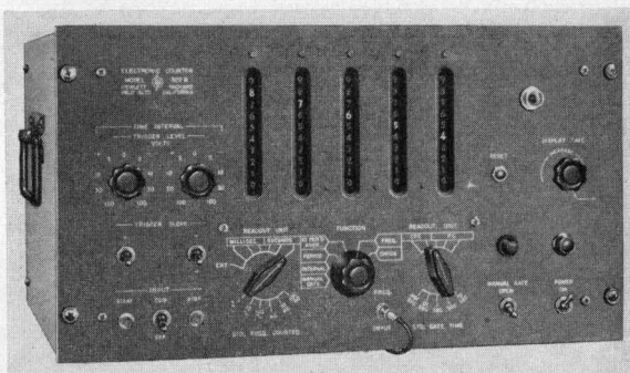
Fig. 1. New -hp- Model 522B Electronic Counter operates up to 100 kc and includes provision for time interval and period measurements.
