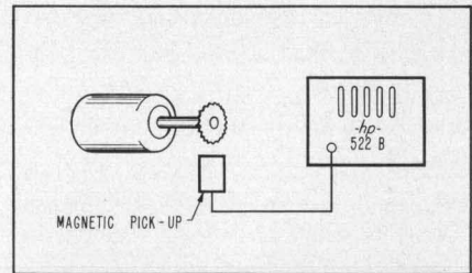
Fig. 4. Set-up for measuring rotation of high-speed shaft.
